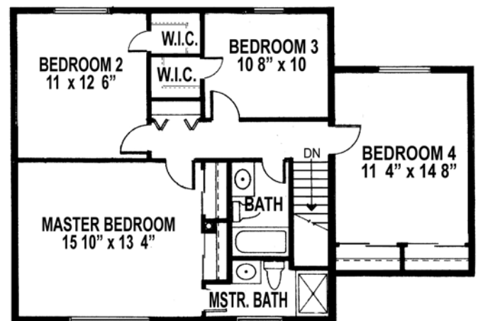
SECOND FLOOR (shown with 4th bedroom)
